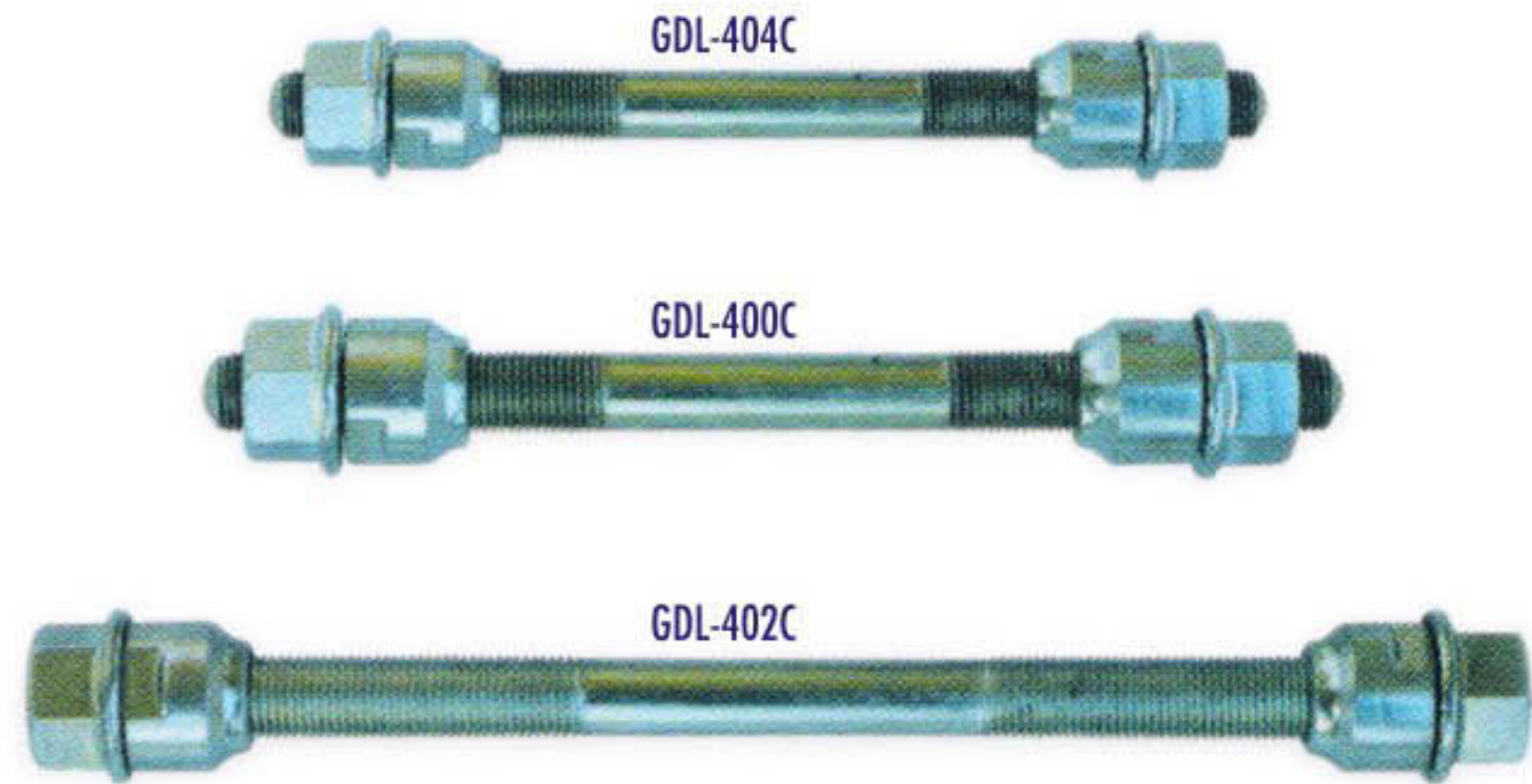
GDL-404C 5/16" x 130mm Packing : 30Doz/ctn N.W/G.W : 29/30kgs Meas : 32x25x21cm GDL-400C 3/8"x 140mm Packing : 20 Doz/ctn N.W/G.W : 29/30kgs Meas : 32x25x21cm GDL-402C 3/8"x 170mm Packing : 20 Doz/ctn N.W/G.W : 32/33kgs Meas : 38x25x21cm
