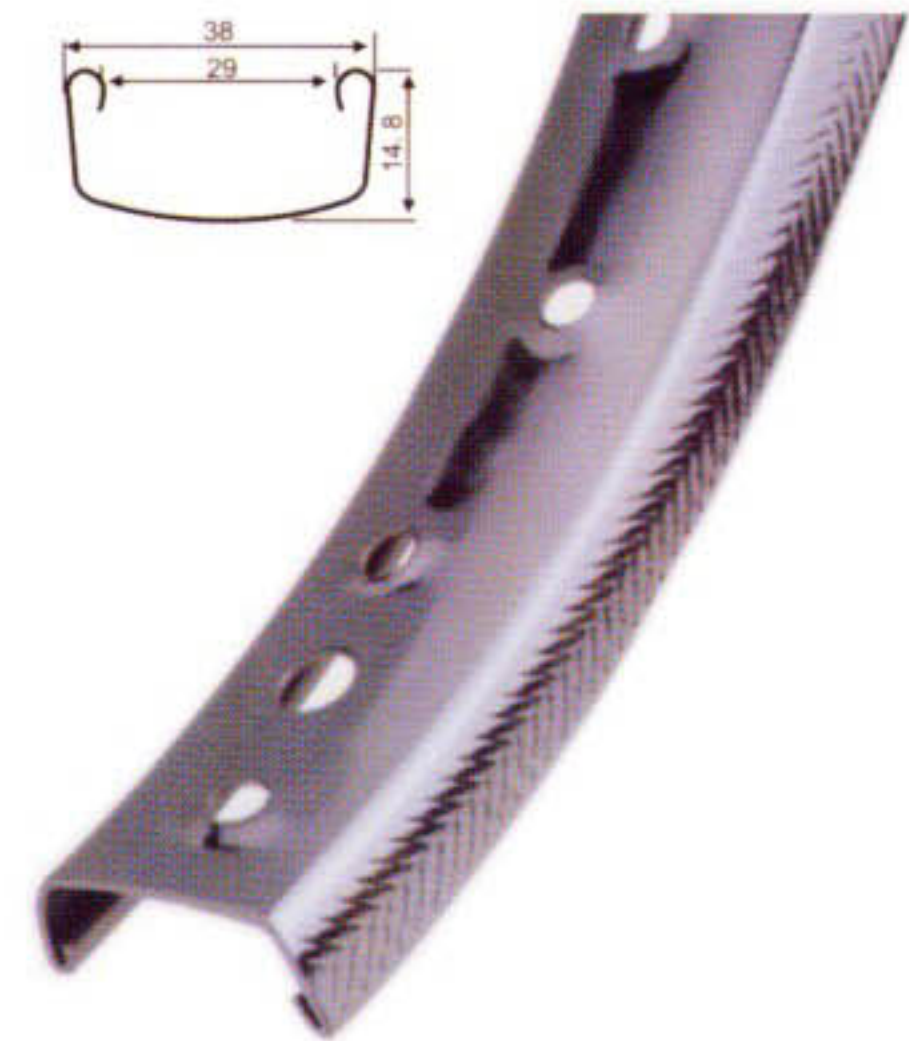
GR-S-010 STEEL RIM Sizes : 12-26" x 2.125 Spoke Holes : 16/20/28/32/36H Finish : CP or ED
