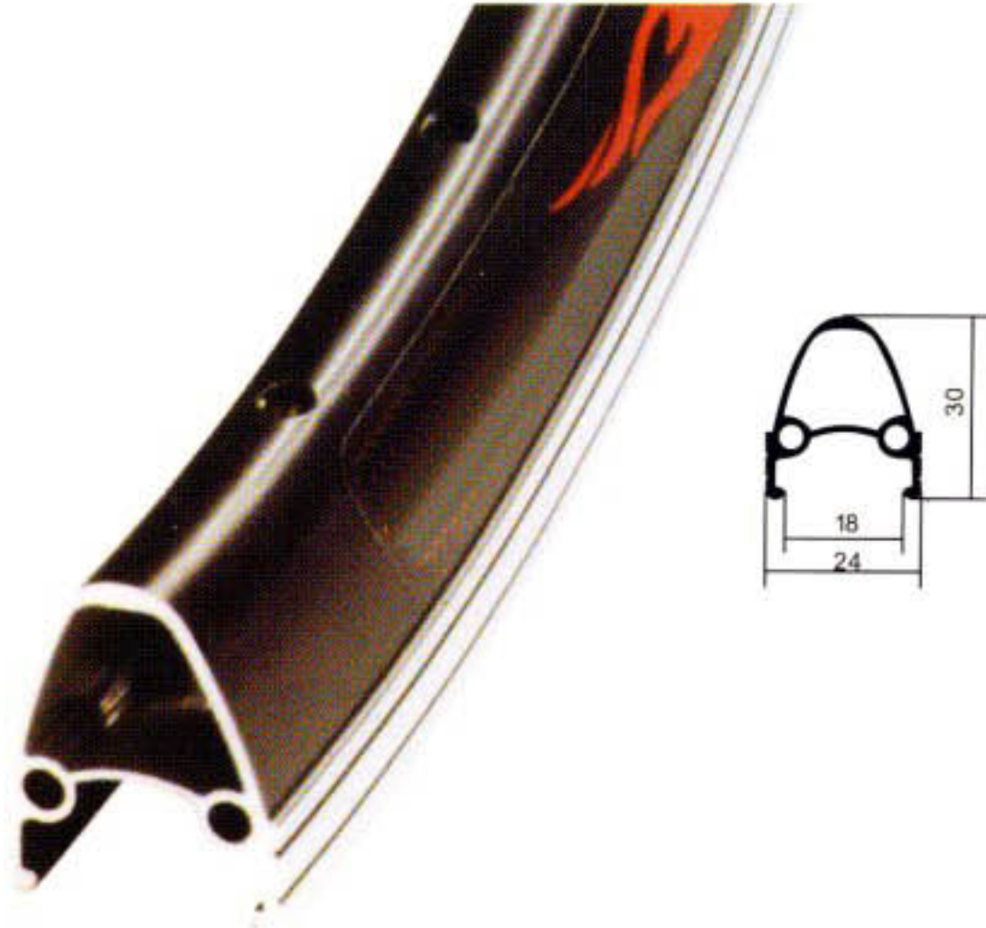
GR-A-024 ALLOY RIM Sizes : 20-26" x 1.75, 22-26" x 1-3/8, 27" x 1-1/4 Spoke Holes : 20/24/32/36H Finish : Painting with CNC side
