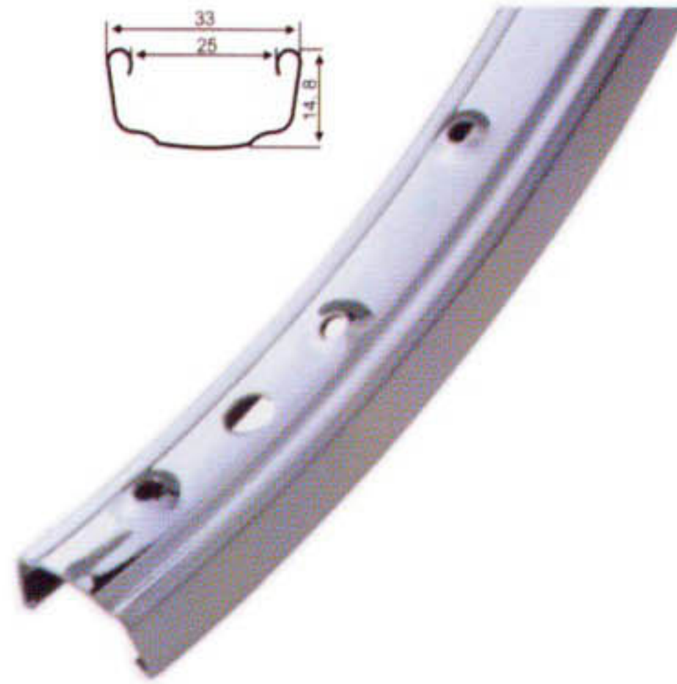
GR-S-007 STEEL RIM Sizes : 12-26" x 1.75-2.125 Spoke Holes : 16/20/28/32/36H(7X profile) Finish : CP or ED
