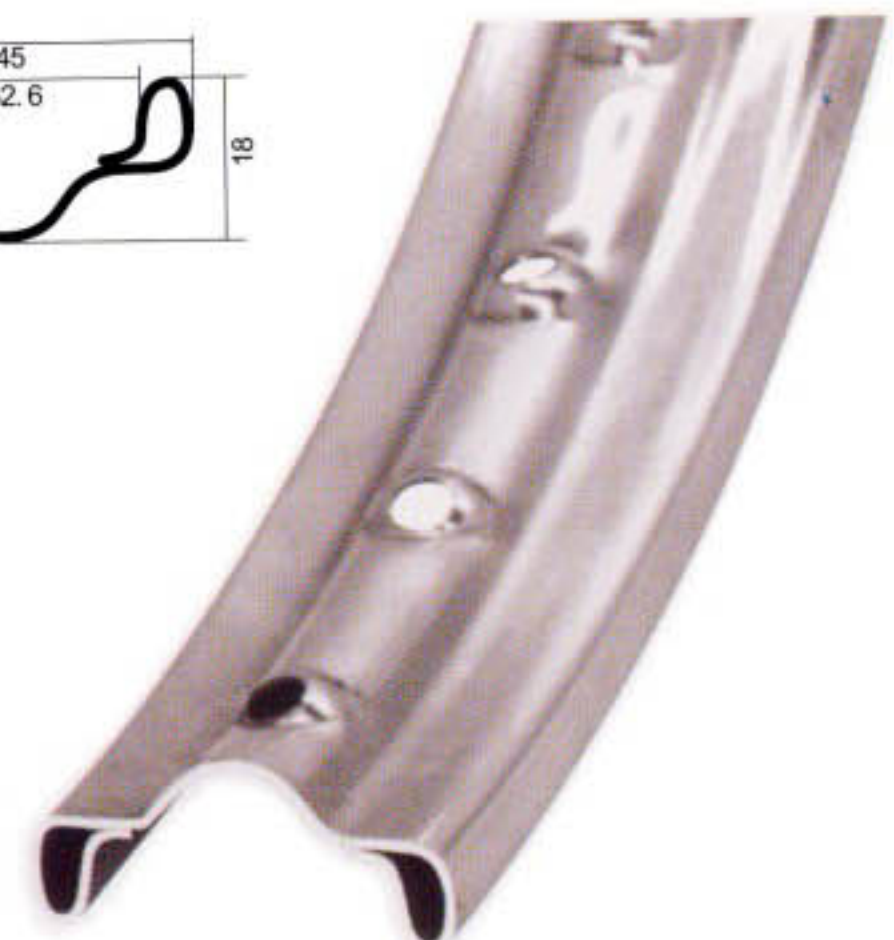
GR-S-022 STEEL TRICICLO RIM Sizes : 26 x 2.00/ 26 x 2.125/ 20 x 2.125 Spoke holes : with dimple 36H Finish : CP or ED
