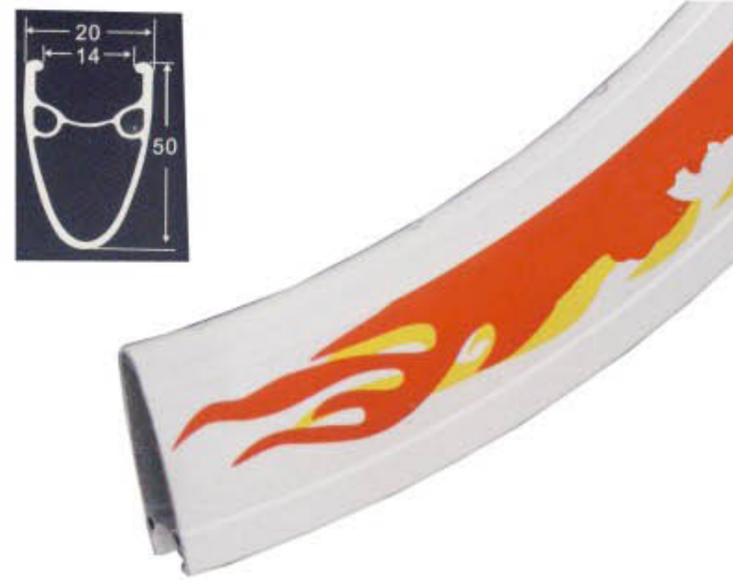
GR-A-S14H50 ALLOY RIM Sizes : 700C Spoke Holes : 32H/36H Finish : Painting
