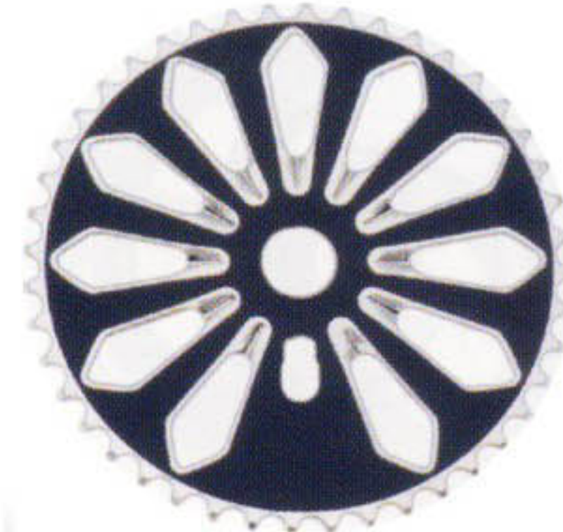
GOPCW-Z116 CHAINWHEEL FOR OPC No. of Teeth : 44/46T Finish : na
