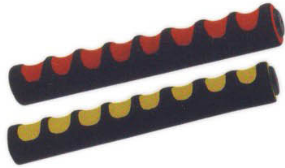
GJSGR-26 GRIP Size : \phi 20x220mm, 4pcs/set Material : Eva with rubber ends
