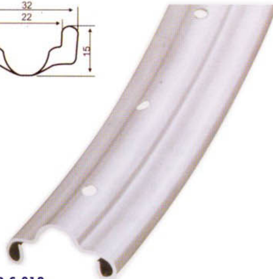
GR-S-012 STEEL RIM Sizes : 24" - 26" x 1-3/8 Spoke Holes : 28H/36H Finish : CP or ED
