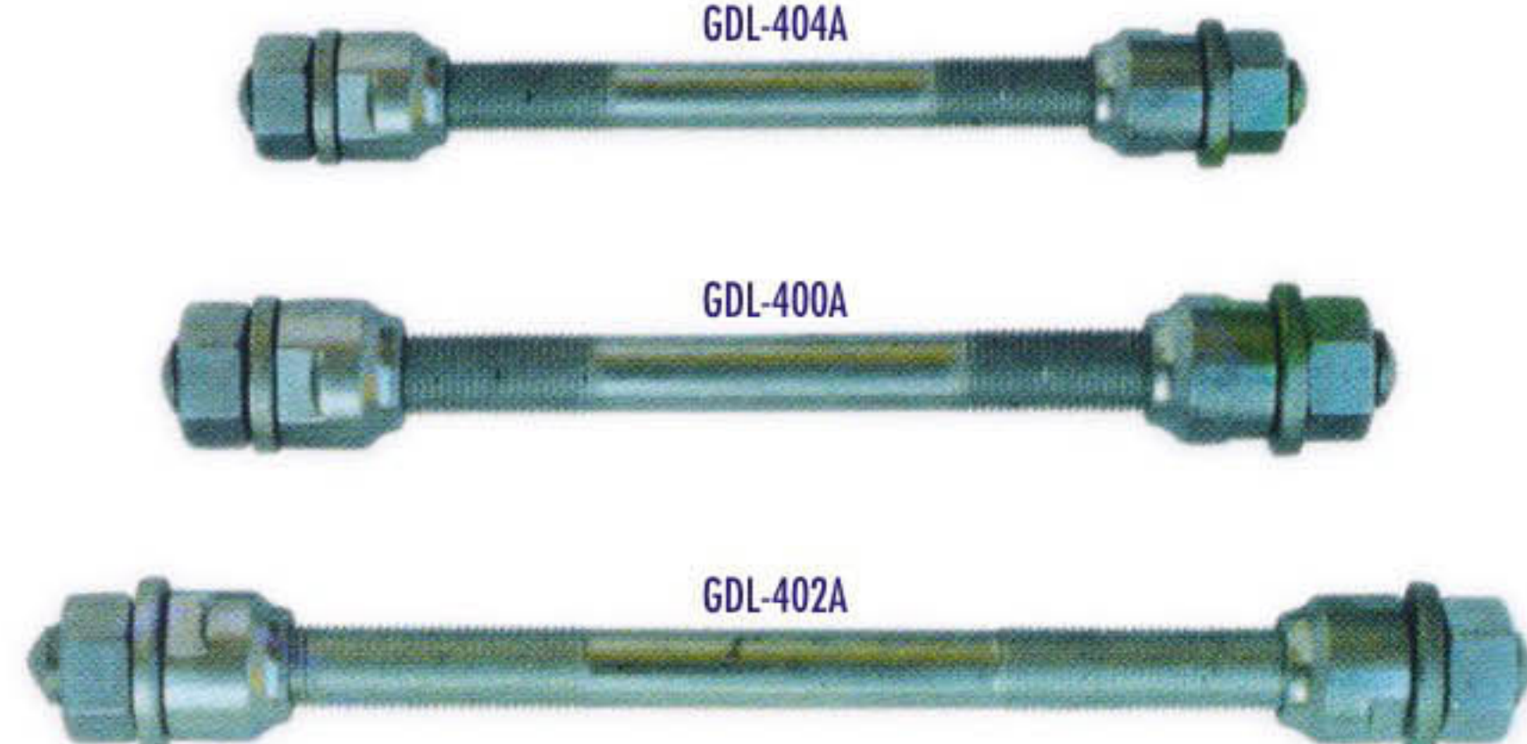
GDL-404A 5/16" x 130mm Packing : 30Doz/ctn N.W/G.W : 28/29kgs Meas : 32x25x21cm GDL-400A 3/8"x 140mm Packing : 20 Doz/ctn N.W/G.W : 29/30kgs Meas : 32x25x21cm GDL-402A 3/8"x 170mm Packing : 20 Doz/ctn N.W/G.W : 32/33kgs Meas : 38x25x21cm
