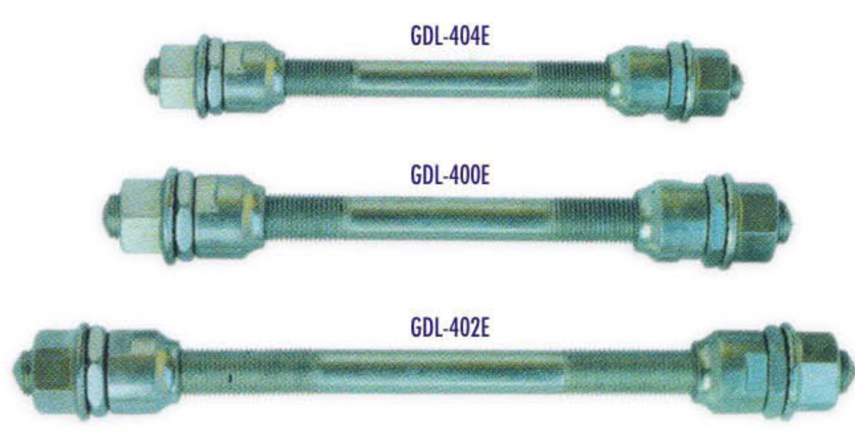
GDL-404E 5/16" x 130mm Packing : 30Doz/ctn N.W/G.W : 32/33kgs Meas : 32x25x21cm GDL-400E 3/8"x 140mm Packing : 20 Doz/ctn N.W/G.W : 32/33kgs Meas : 32x25x21cm GDL-402E 3/8"x 170mm Packing : 20 Doz/ctn N.W/G.W : 34/35kgs Meas : 38x25x21cm
