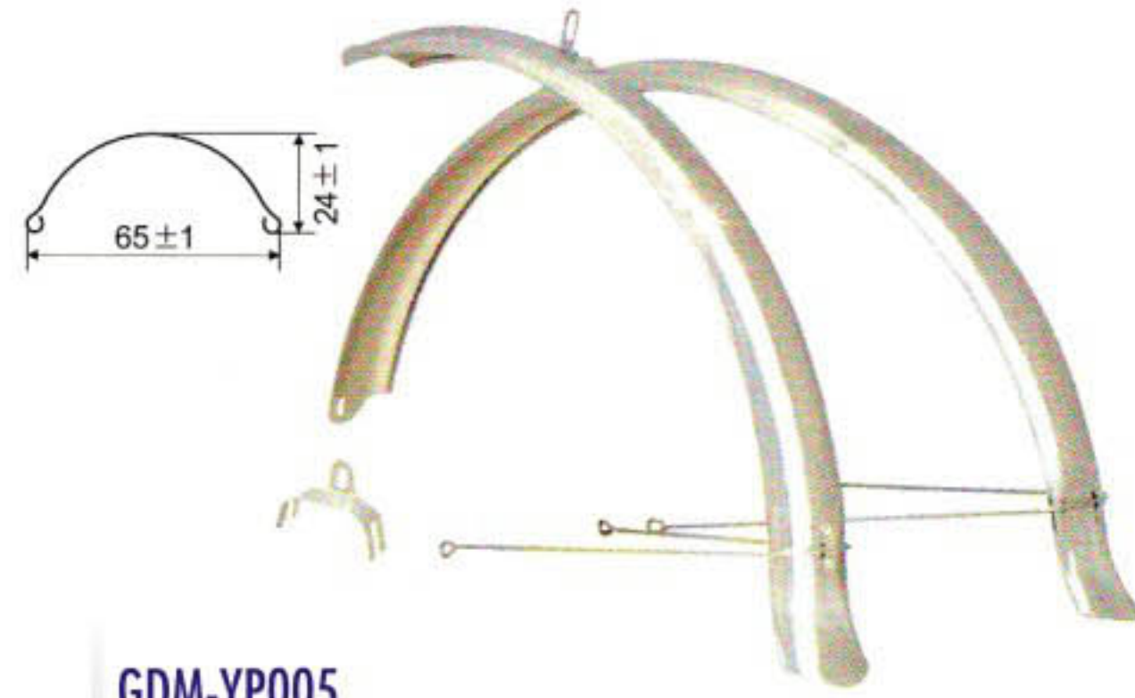
GDM-YP005 MUDGUARD Material : STEEL/STAINLESS Size : 1.95~2.125 Packing : 26": 76X46X32=50PRS 37.5/36.5
