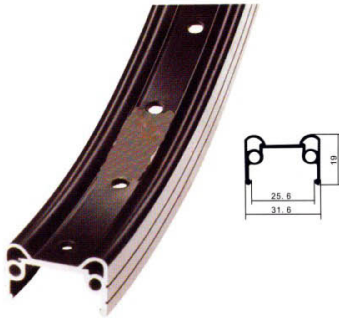
GR-A-028 ALLOY RIM Sizes : 16-24" x 1.75 Spoke Holes : 36/48/68H Finish : Painting with CNC side
