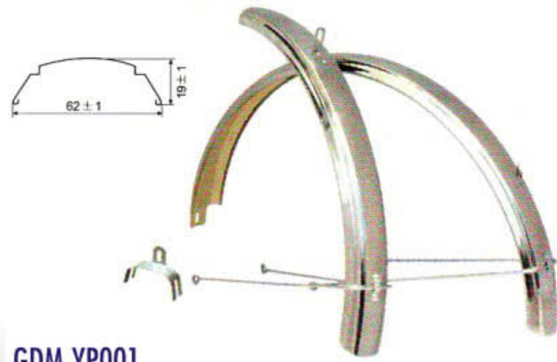
GDM-YP001 MUDGUARD Material : STEEL/STAINLESS/ALLOY Size : 20"/24"/26"X2.125 Packing : 26": 76X46X32=50PRS 37.5/36.5
