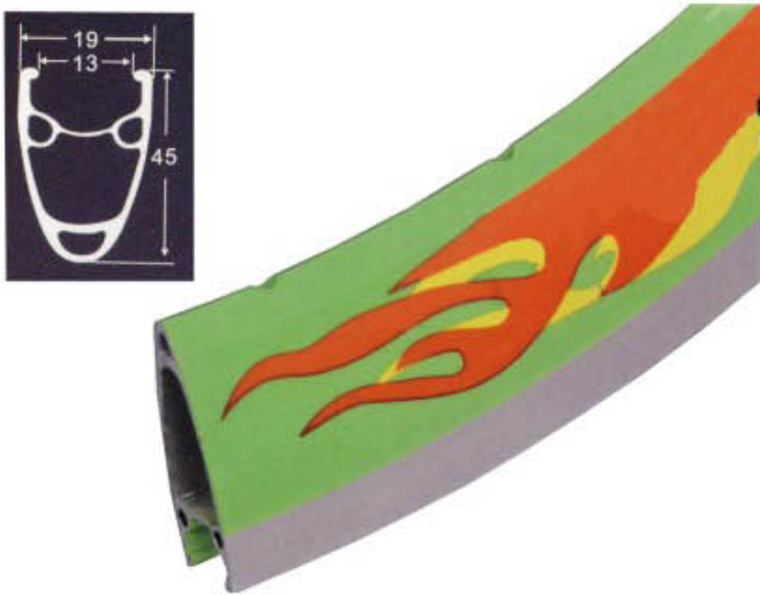
GR-A-S13H45 ALLOY RIM Sizes : 26 x 1.00 - 1.5 (650C and 700C) Spoke Holes : 32H/36H Finish : Painting
