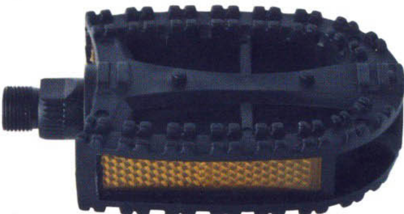
GPN-B118 CHILDREN NYLON FOOT PEDAL Size : 110mm x 65mm Finish : Black/ Colors
